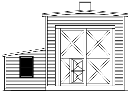
North Elevation
