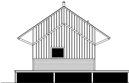
North Elevation
