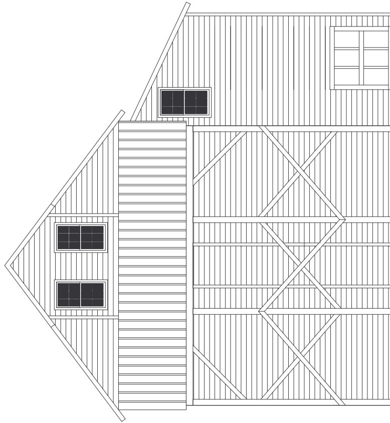
North Elevation
